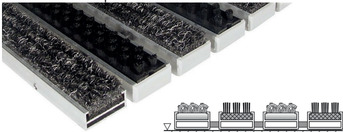
brush strip 3 / 2x textile
