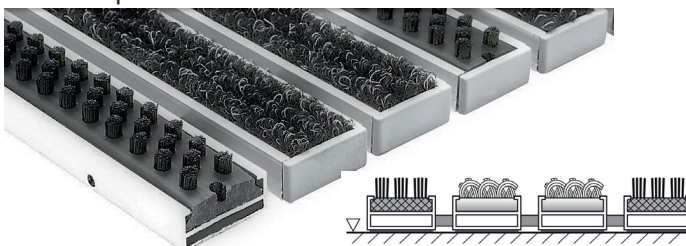
grooved PVC / Y-shaped aluminium
